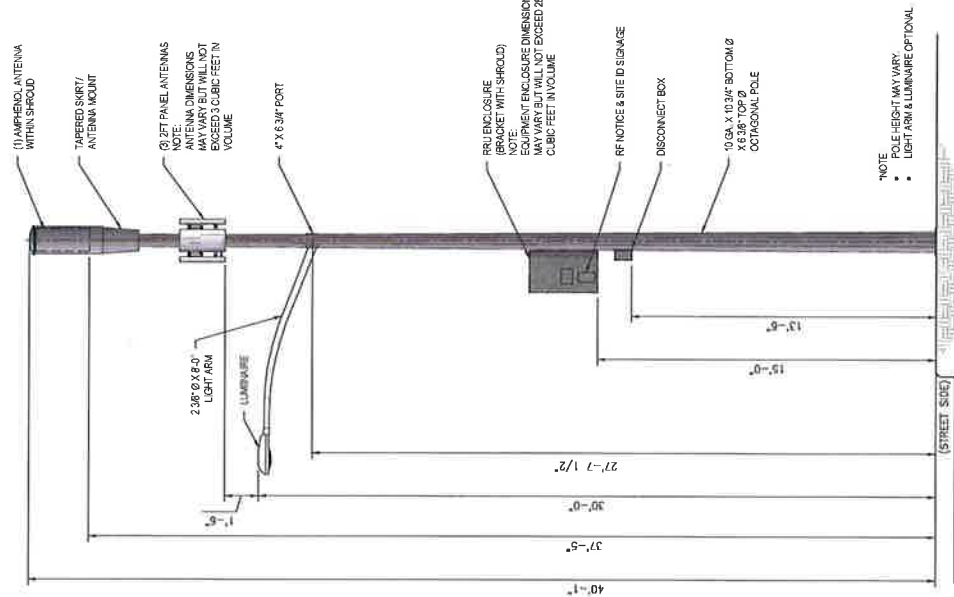
Elevation Profile
